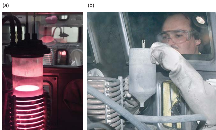
Figure 3. Cast Plutonium
